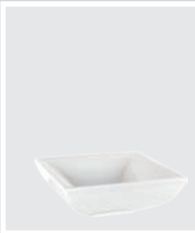
450 x 450 x 156 h mm 37503 with overflow waste 37504
